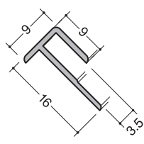
F型出隅 (W形状)
