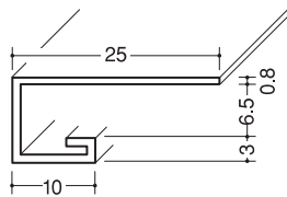
AG-7S 2m/2.3m(取寄品)
