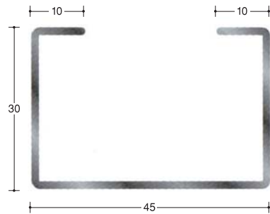
補強材45 3m・6本束
