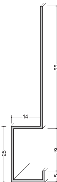
DX-1914 (CK-1) 3m, 20本入
