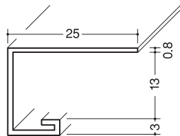
AG-13S 2m/2.3m(取寄品)
