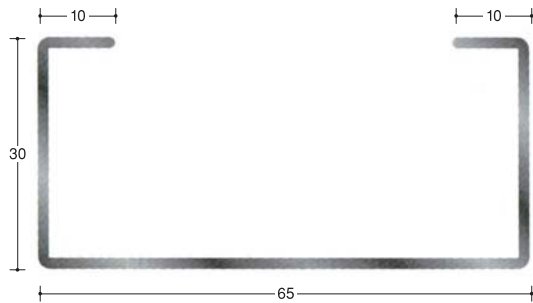
補強材65 3m・6本束
