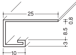
AG-8.5S 2m/2.3m(取寄品)
